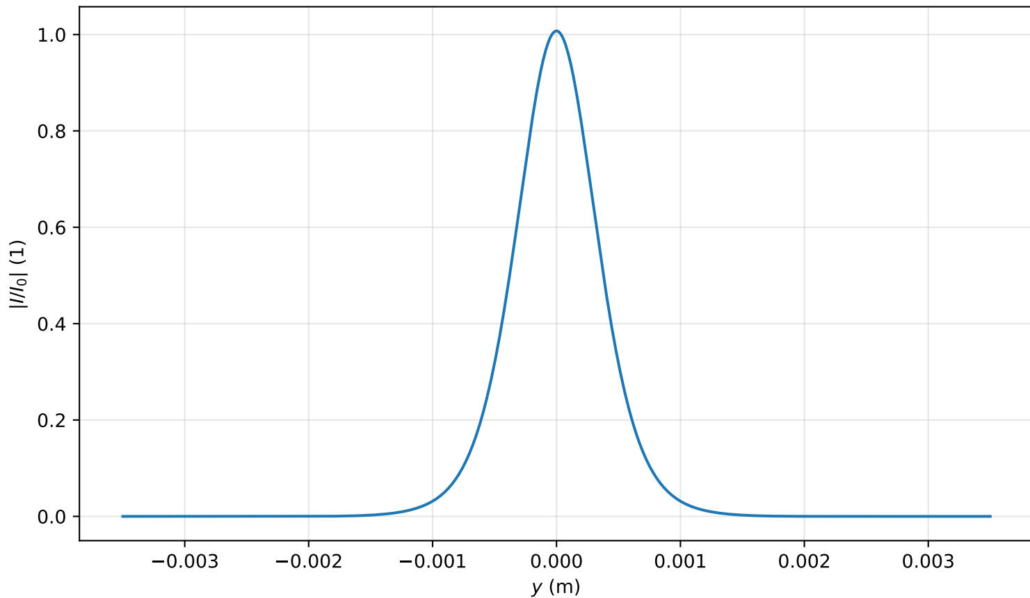
Intensity profile I(x=0, y, z=1.751)/I_0 , P_{in}=0.6P_{cr} , artificial time
